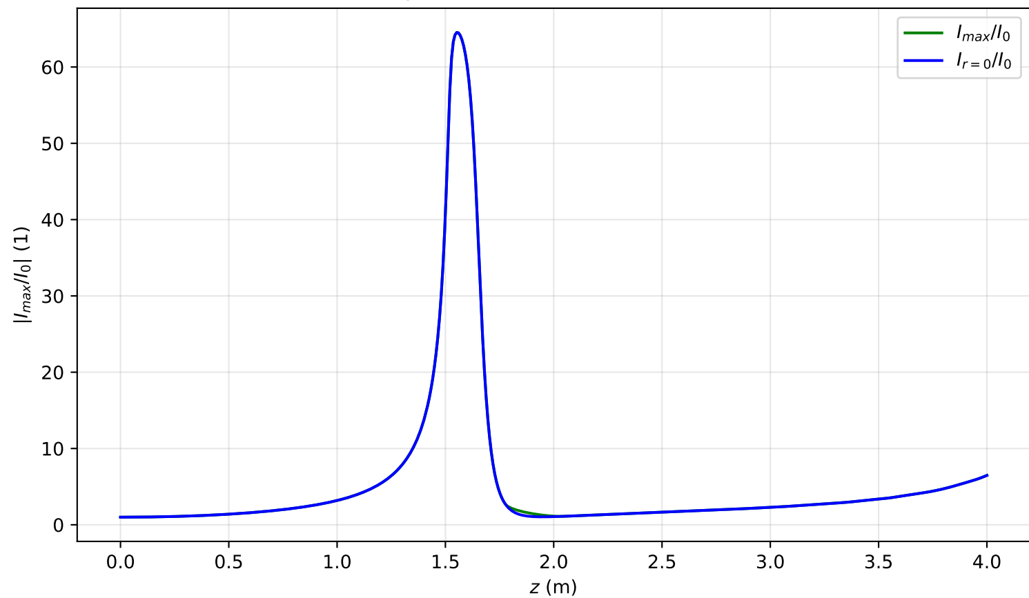
I_{max}(x = 0, y = 0, z)/I_0 , Pin=1.6P_{cr} , artificial time
